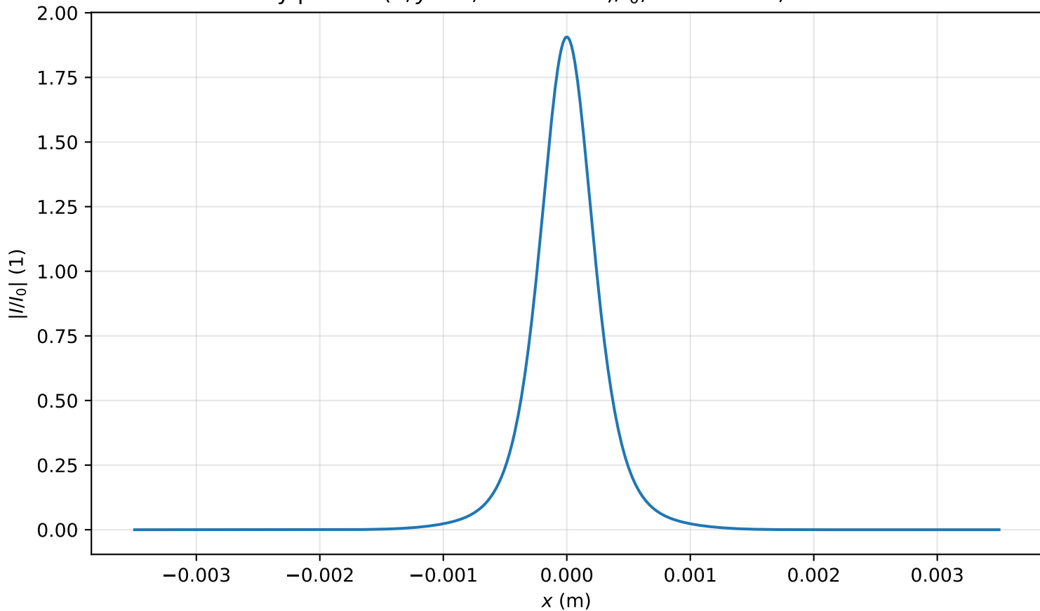
Intensity profile I(x, y = 0, z = 1.592m)/I_0 , P_{in}=1.0P_{cr} , artificial time
